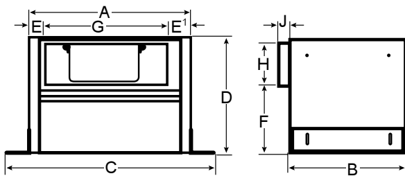
Figure 15: Models Z3H, Z5H and Z6S/H
