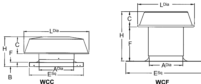
Figure 13: Weather Caps
