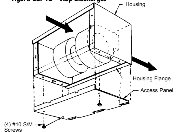
Figure 29: "TD" (Top Discharge)
