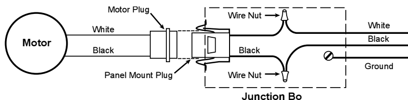
Figure 6: Internal Electrical Connections, Single Speed Motors
