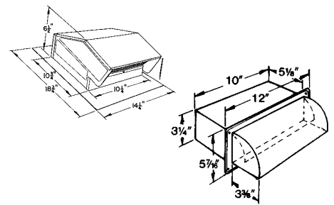
Figure 10: Duct Transitions
