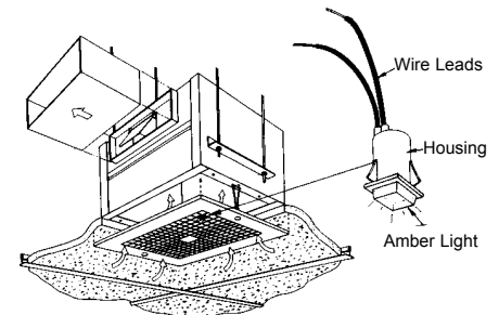
Figure 11: Pilot Light
