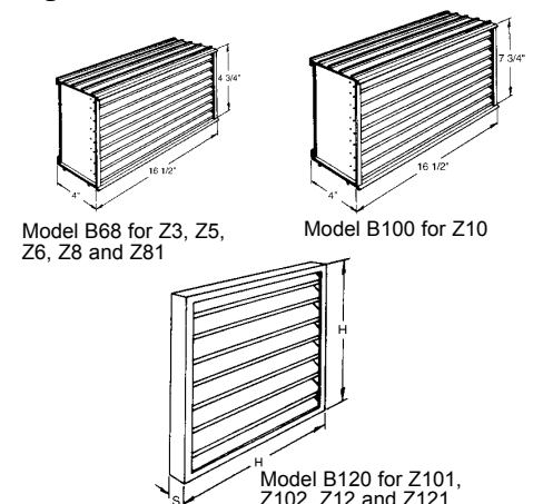
Figure 12: Brick Vents
