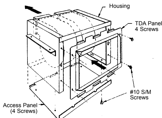
Figure 30: "TDA" (In-Line)
