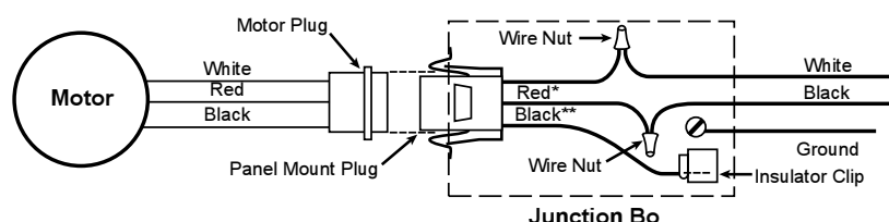
Figure 7: Internal Electrical Connections, Two Speed Motors
