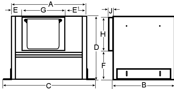
Figure 16: Models Z8S/H AND Z81S
