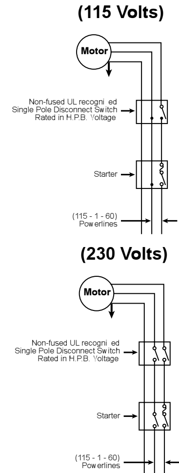
Figure 8: External Electrical Connections
